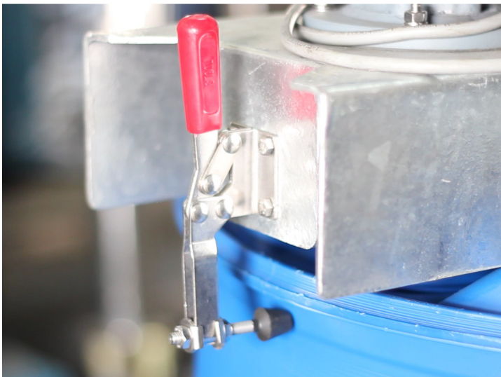
Figure 5: Safety mechanism with clamping and limit switches.
